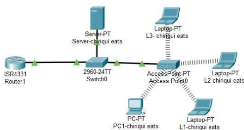
Diagrama de packet tracer
